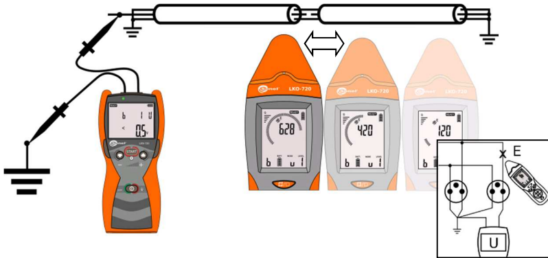
Fig. 25 Locating breaks.
