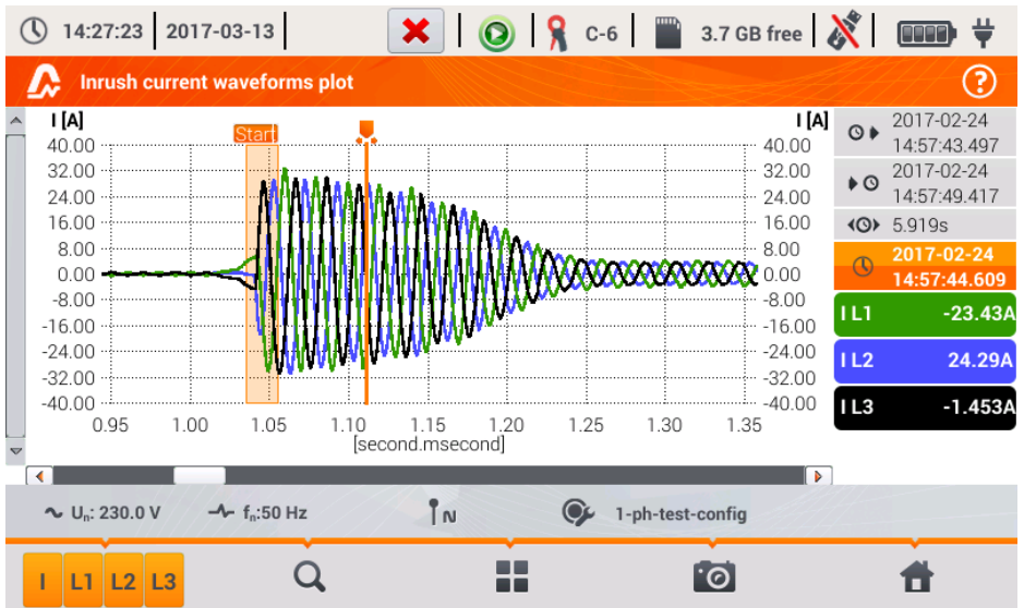
Fig. 38. Inrush current analysis – waveforms plots.
