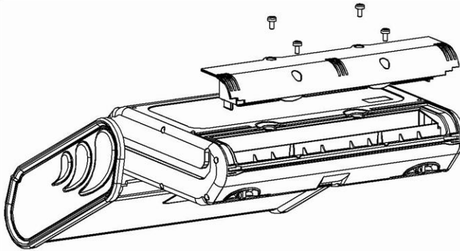
Fig. 75. Replacing the battery pack
