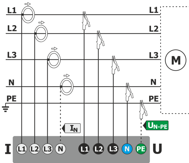
Fig. 49. Wiring diagram – 3-phase 4-wire system.
