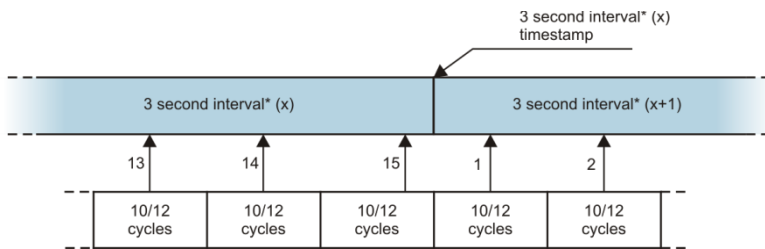
Fig. 65. Determining the averaging intervals shorter than 10 seconds (with the 3-second averaging).
