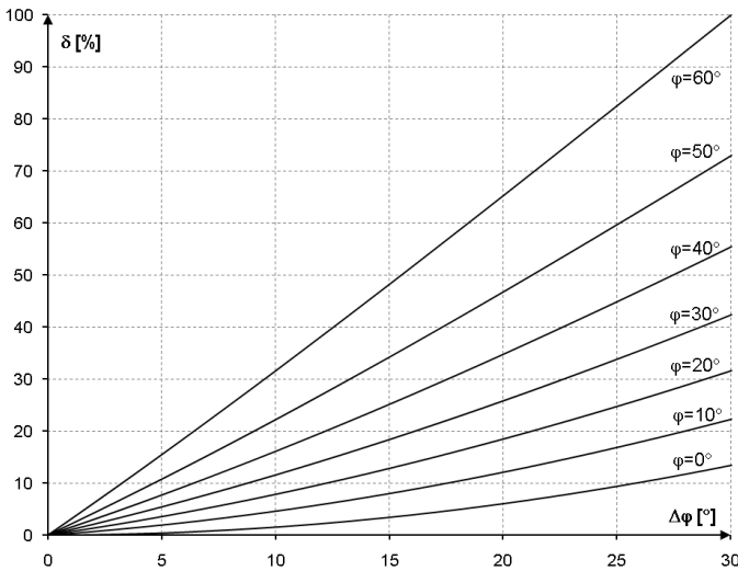
Fig. 67. Additional uncertainty from phase error depending on phase shift angle.
