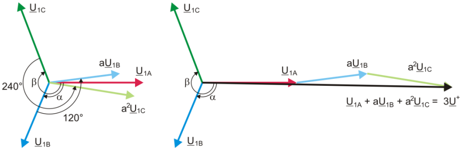
Fig. 60. Example of determination of positive sequence component.
