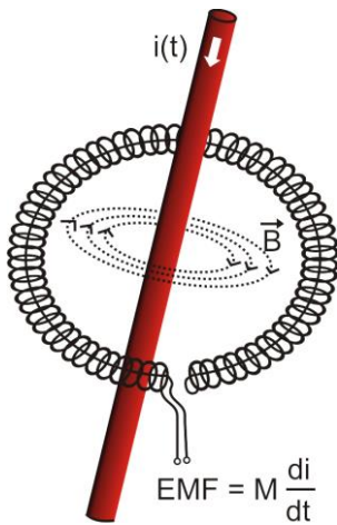
Fig. 59. Rogowski coil.
