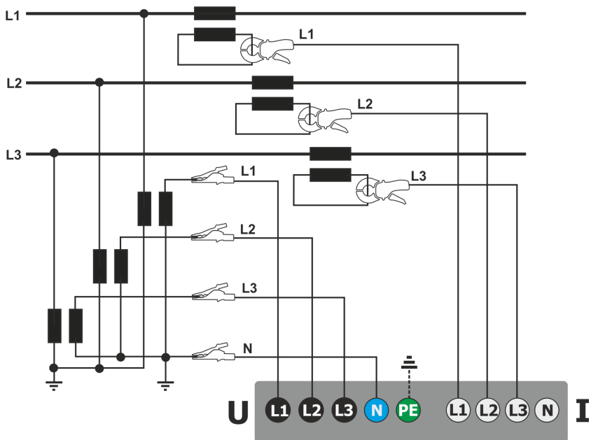
Fig. 52. Wiring diagram – indirect measurement of MV in 3-phase 4-wire system.
