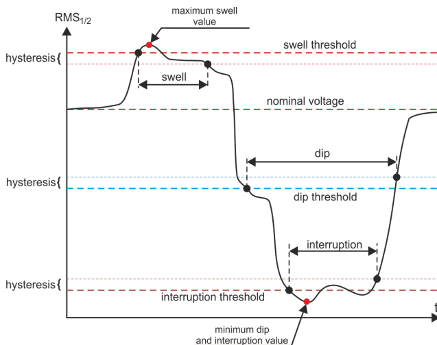
Fig. 61. Voltage swells, dips and interruptions.
