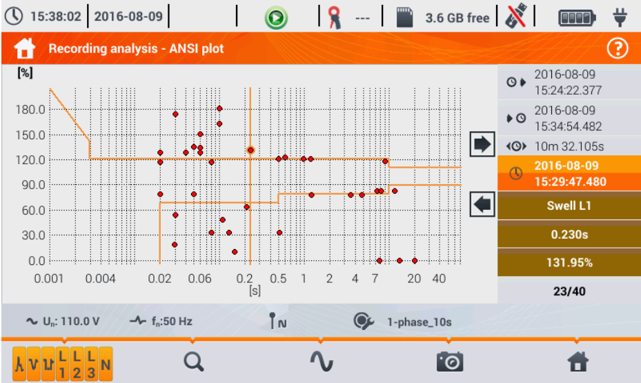
Fig. 30. Recording analysis – ANSI graph.
