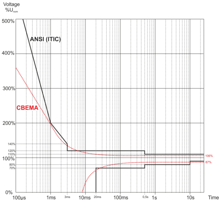
Fig. 63. Voltage tolerance curves ANSI (ITIC) and CBEMA.
