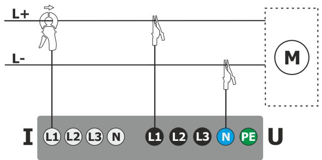
Fig. 54. Wiring diagram – DC system.
