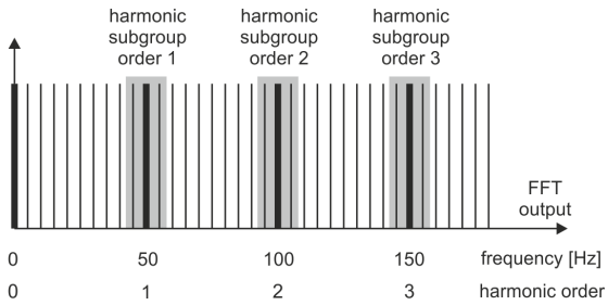
Fig. 57. Determination of harmonic subgroups (50 Hz system).
