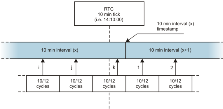
Fig. 64. Determining the averaging intervals equal to or longer than 10 seconds (with the 10-minute averaging).
