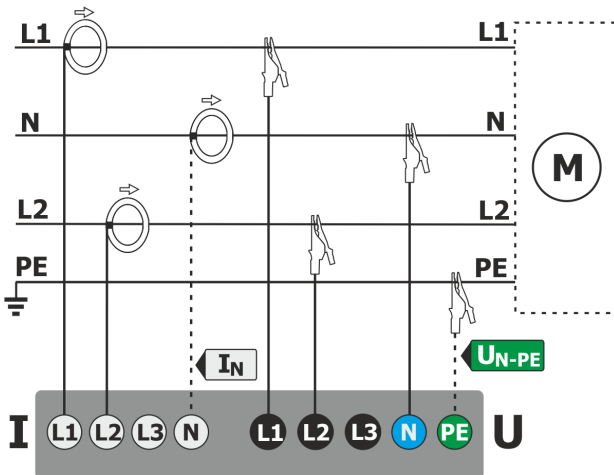
Fig. 48. Wiring diagram – split-phase.
