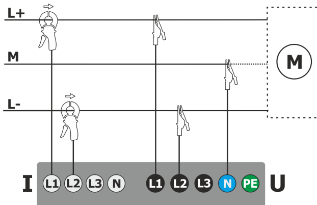
Fig. 55. Wiring diagram – DC+M system (bipolar).
