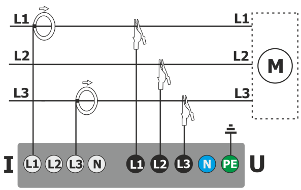
Fig. 51. Wiring diagram – 3-phase 3-wire system (current measurement using Aron method).
