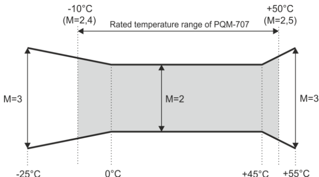
Fig. 66. Basic uncertainty multiplier M as a function of ambient temperature (does not apply to the reference conditions).
