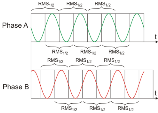
Fig. 62. Determination of the U_{rms(1/2)} value.
