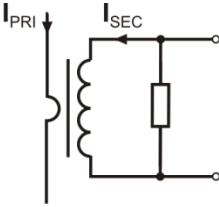
Fig. 58. Current transformer clamp with voltage output.
