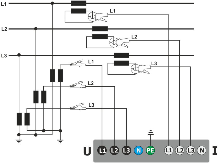
Fig. 53. Wiring diagram – indirect measurement of MV in 3-phase 3-wire system.
