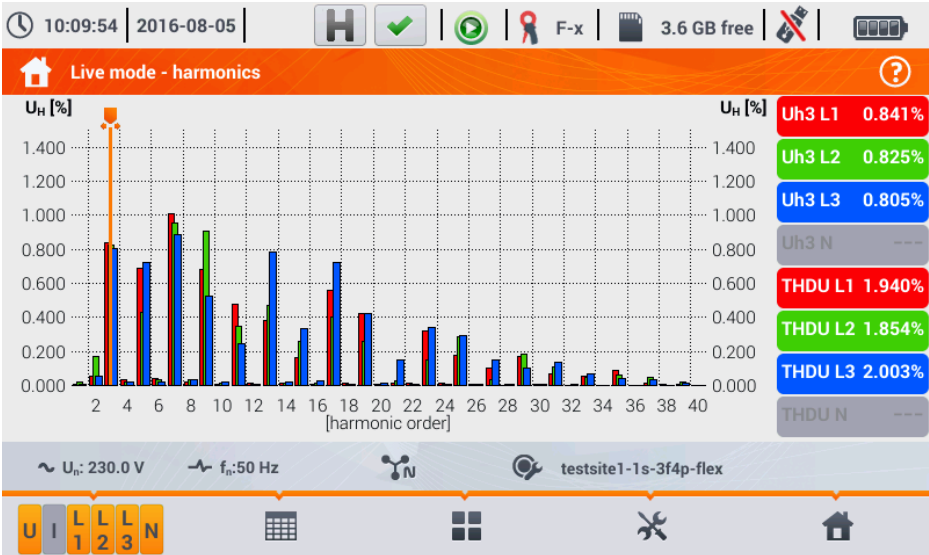
Fig. 45. Live mode - harmonics - bar graph.
