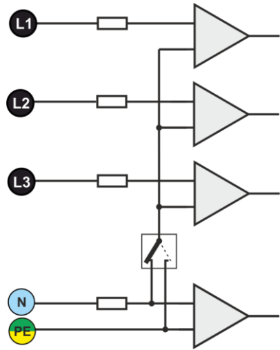
Fig. 56. Voltage input terminals
