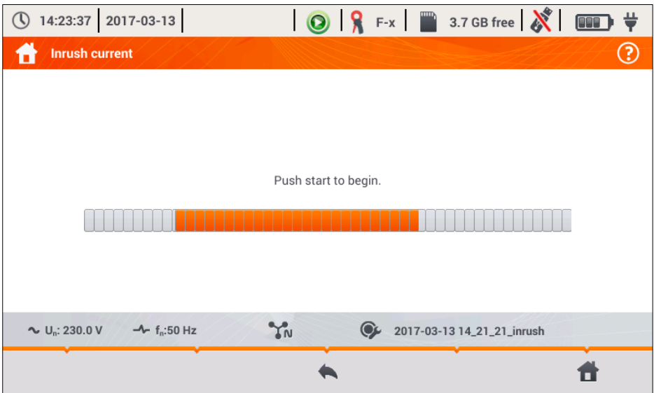
Fig. 36. Inrush current - waiting for start of the measurement.
