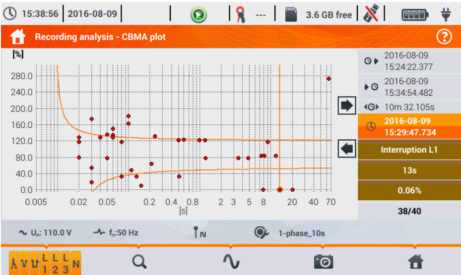
Fig. 31. Recording analysis - CBEMA graph.
