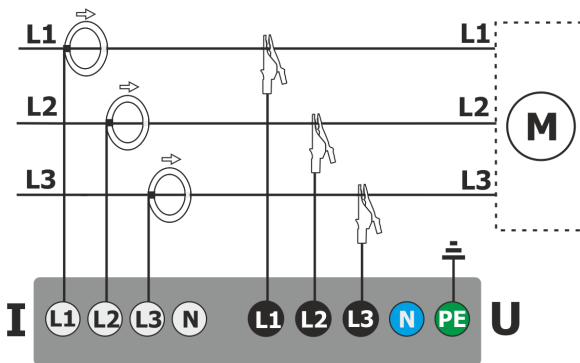
Fig. 50. Wiring diagram – 3-phase 3-wire system.
