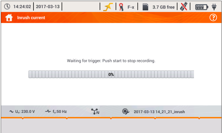
Fig. 37. Inrush current - waiting for triggering the measurement.
