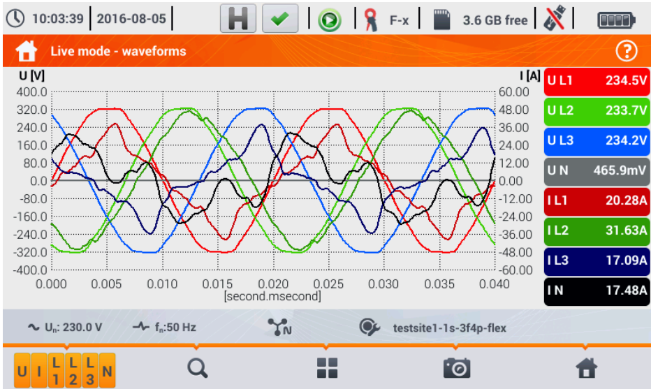
Fig. 41. Current readings - waveforms.
